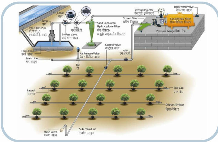
DRIP IRRIGATION SYSTEM
