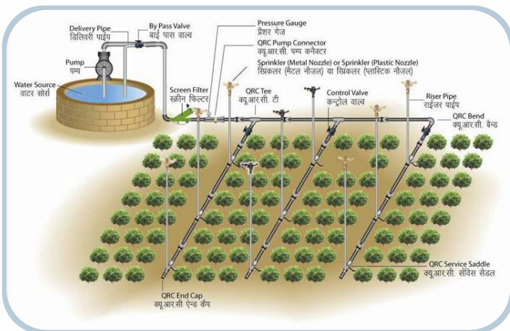
SPRINKLER IRRIGATION SYSTEM
